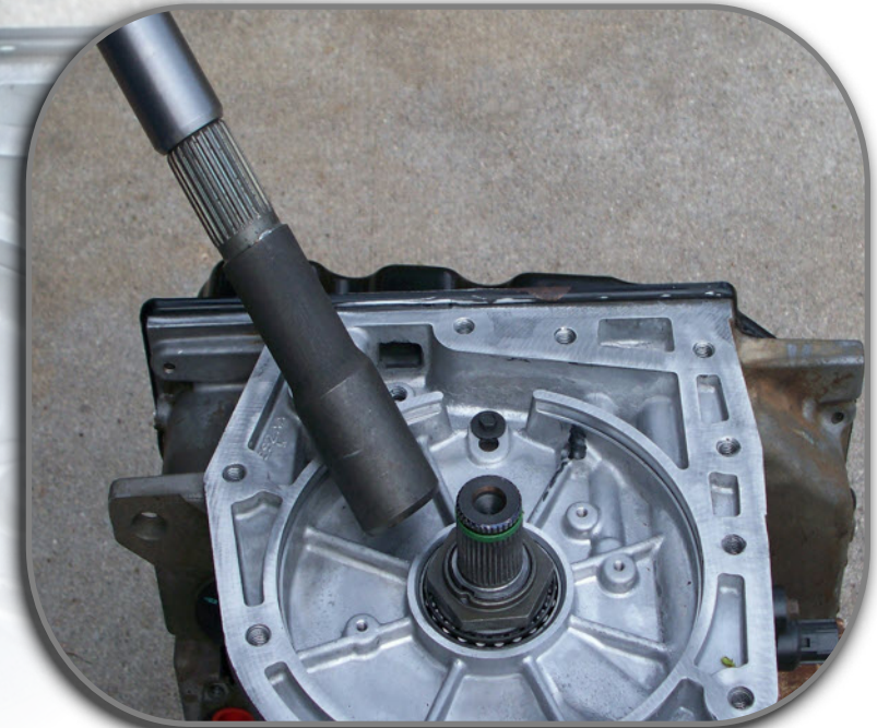
▲ Note the green circlip on the splined shaft.
